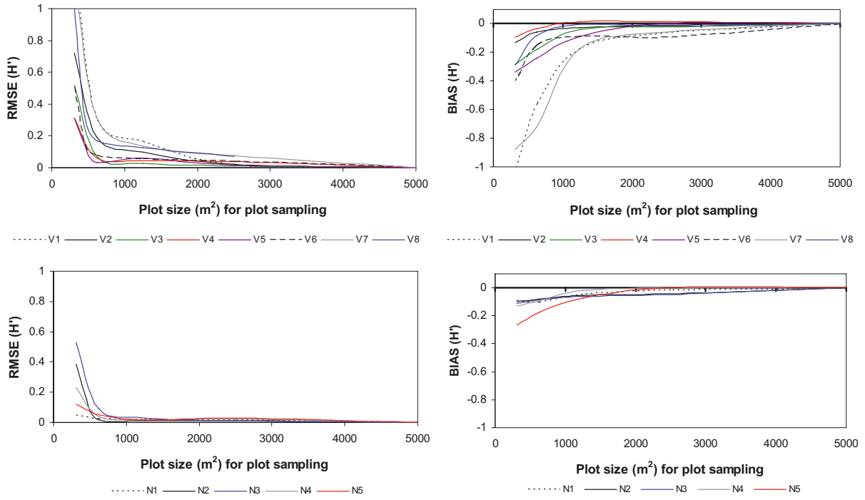
Figure A.3. RMSE and Bias statistics in relation to the plot size for the estimated values of the non-spatially explicit index H' , in Valsain (V1–V8) and Navafria (N1–N5).
