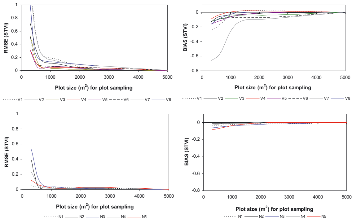
Figure A.1. RMSE and Bias statistics in relation to the plot size for the estimated values of the non-spatially explicit index STVI, in Valsain (V1–V8) and Navafria (N1–N5).
