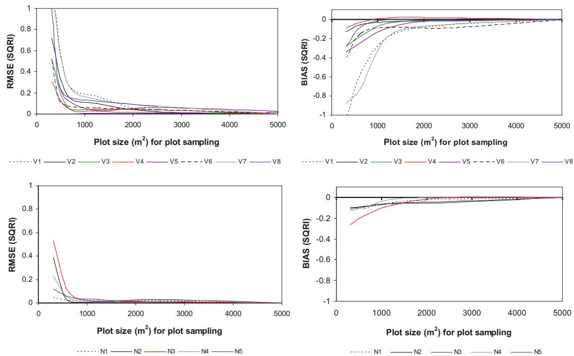
Figure A.2. RMSE and Bias statistics in relation to the plot size for the estimated values of the non-spatially explicit index SQRI, in Valsain (V1–V8) and Navafria (N1–N5).
