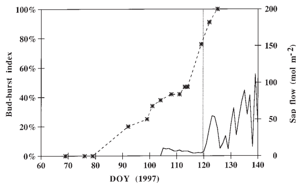
Figure 2. Variation of bud-burst index (asterisks) and sapflow (solid line) during the early period of 1997 growing season. The bud-burst index is ranged from 0 to 100. The threshold for the beginning of the growing season 1997 is shown and indicates the date (DOY 120) at which starts calculation for carbon balance.
