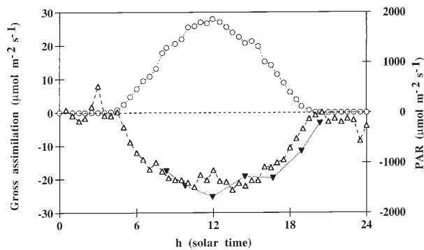
Figure 5. Diurnal pattern on DOY 190 of radiation and estimates of gross assimilation. The symbols represent the incoming photosynthetically active radiation (circles), gross assimilation calculated from eddy covariance measurements (triangles) and gross assimilation derived from measurements using Li-Cor 6200 on 5 trees scaled to the stand (inverted triangles). Data are averaged according to time of day.
