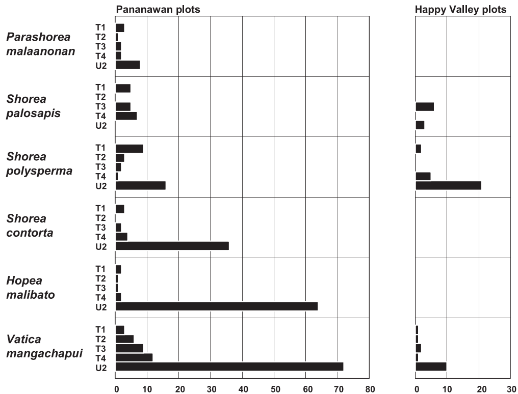
Figure 4. Representation of the six most common dipterocarp species in five height layers distinguished in the “Pananawan” and “Happy Valley” plots. Individuals encountered in 57 plots; layers T1–T4 represent 100 m 2 plots, U2 subplots of 25 m 2 ; T1: dominant tree layer, T2: > 2/3 of the stand height but not yet being dominant, T3: > 1/3 – 2/3 of the stand height, T4: > 2.5 m – 1/3 of the stand height, U2: > 0.5 m – 2.5 m.
