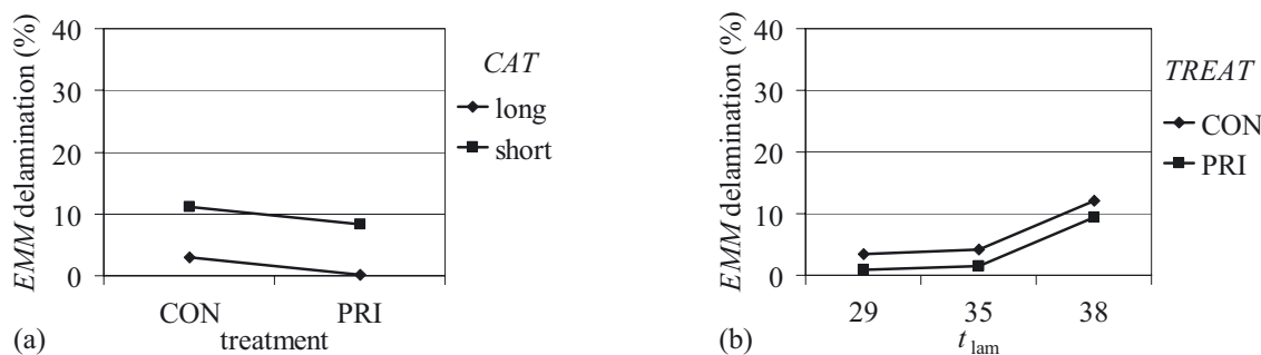
Figure 3. (a) Estimated marginal means ( EMM ) of delamination regarding pre-treatment ( TREAT : PRI = primed; CON = unprimed control) and closed assembly time ( CAT ), irrespective of the lamella thickness ( t_{lam} ). (b) EMM of delamination regarding t_{lam} and TREAT , irrespective of CAT .
